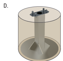
In-Ground Prefabricated anchor PART: 66TOW-EMER-01-304
