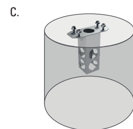
Poured Concrete Prefabricated anchor PART: 66TOW-EMER-02-304
